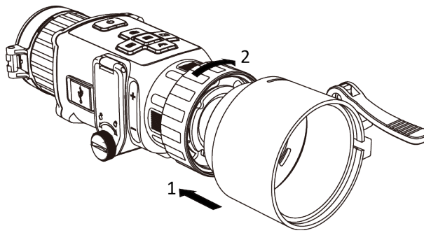
Figure 2-4 Install Adapter
