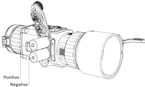
Figure 2-3 Install Batteries
