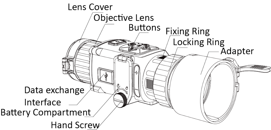
Figure 1-2 Interfaces of Device
