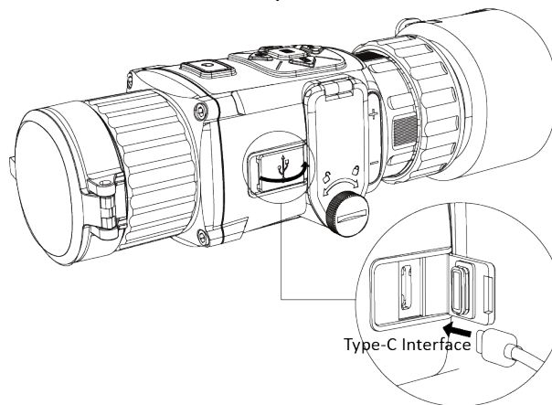
Figure 2-1 Cable Interface
